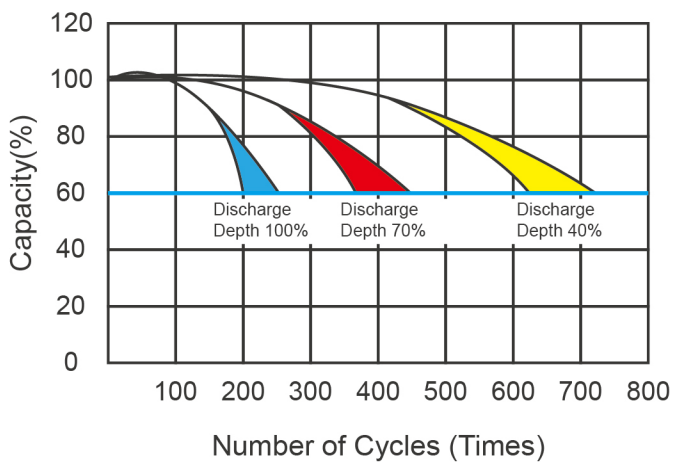
Cycle Service Life (@25°C/77°F)
